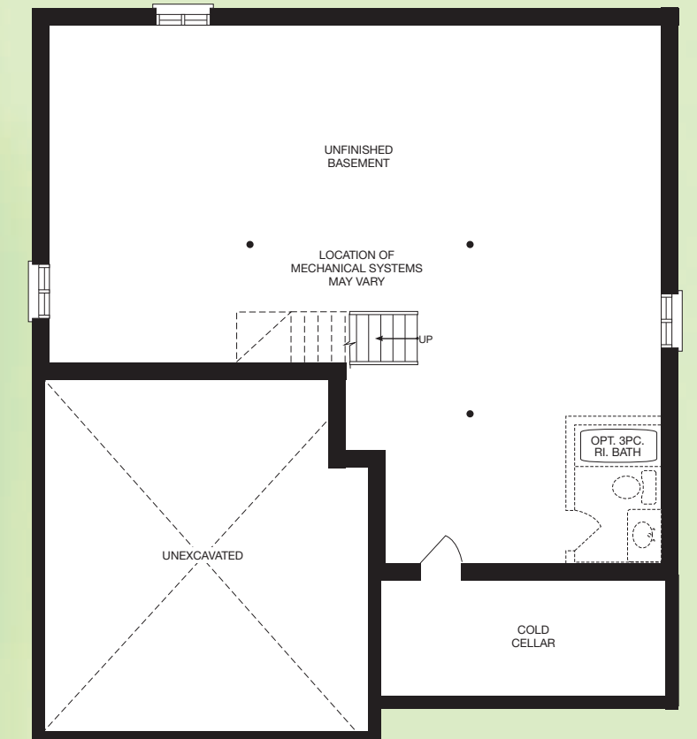
BASEMENT ELEV. A
