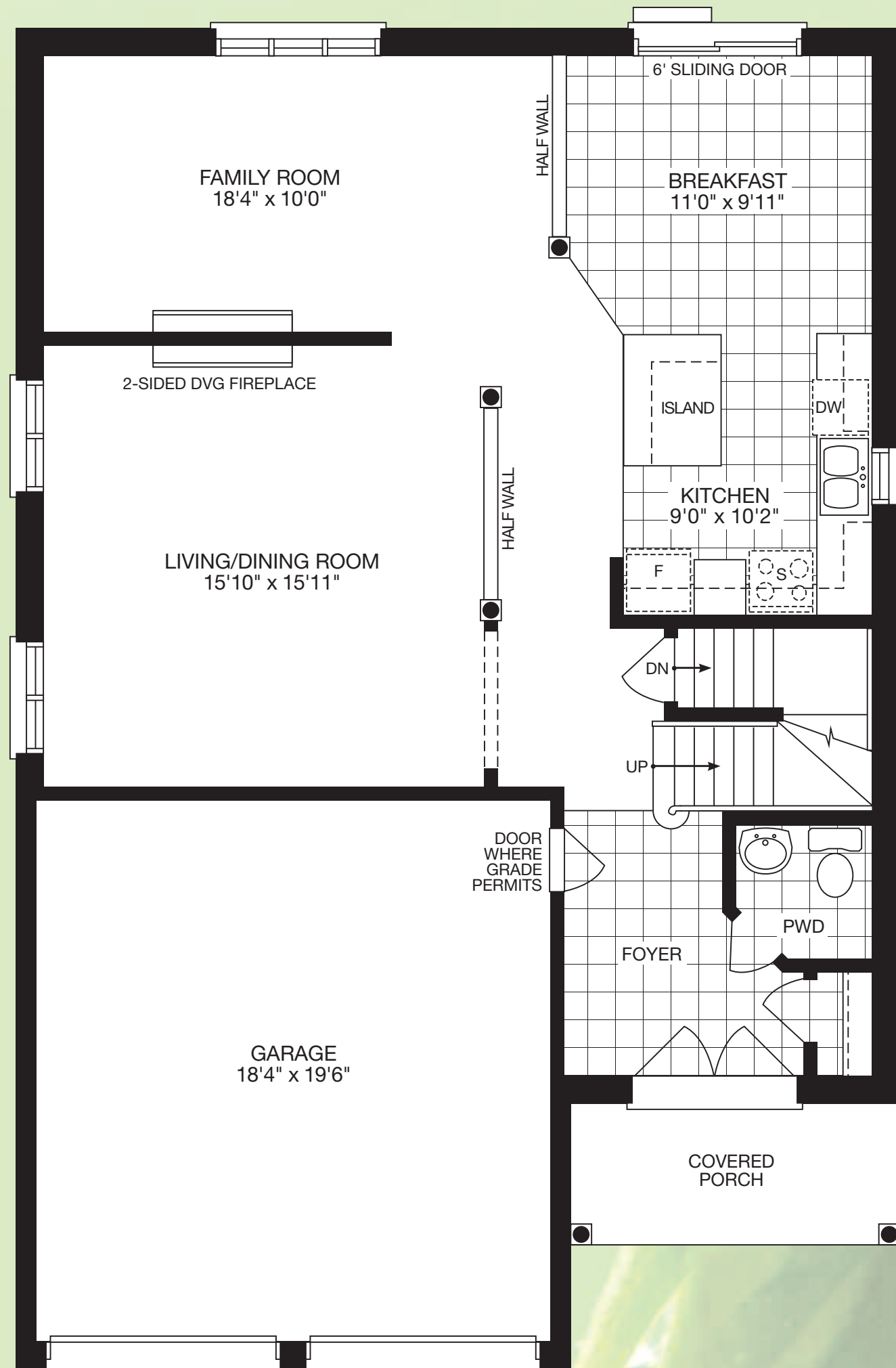
FIRST FLOOR ELEV. A
